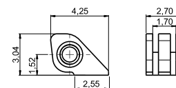
SOLDERING HINGE 03FR27220000
