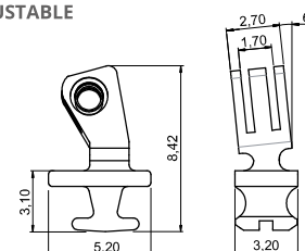
90° INSERT HINGE 03FRC5912A2BN0
