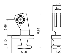
90° INSERT HINGE 03FRC5911A2BN0
