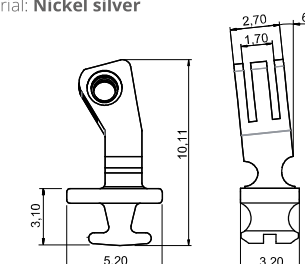
90° INSERT HINGE 03FRC5906A2BN0
