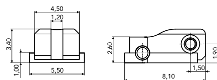
180° FRONT HINGE 03FRA0167A1BN0
