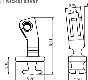
90° INSERT HINGE 03FRC5906A2BN0
