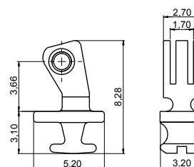
90° INSERT HINGE 03FRC5911A2BN0
