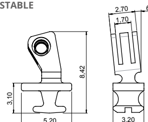
90° INSERT HINGE 03FRC5912A2BN0
