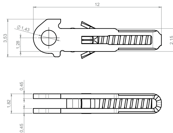
TROLLEY 07CRA0940A1BYX Material: Stainless steel
