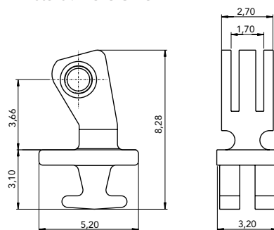
90° PLASTIC HINGE 03FR27222000
