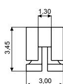
180° PLASTIC HINGE 03FRC4144A2BN0
