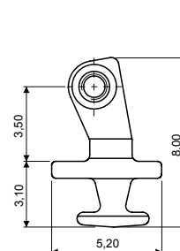
90° PLASTIC HINGE 03FRC4135A2BN0
