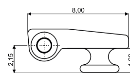
180° PLASTIC HINGE 03FRC4146A2BN0
