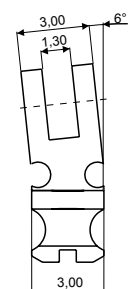
90° PLASTIC HINGE 03FRC4138A2BN0
