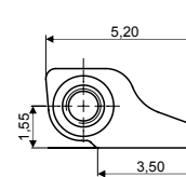
SOLDERING HINGE 03FRC4550A1BY0
