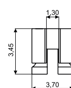
180° PLASTIC HINGE 03FRC4145A2BN0
