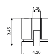
180° PLASTIC HINGE 03FRC4146A2BN0
