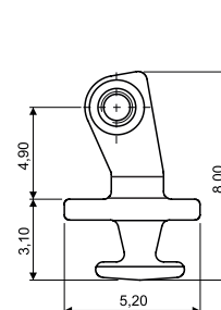
90° PLASTIC HINGE 03FRC4139A2BN0
