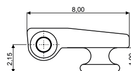
180° PLASTIC HINGE 03FRC4143A2BN0
