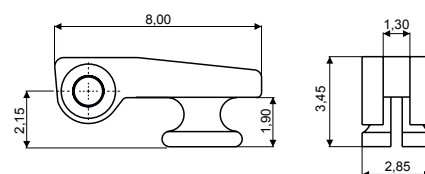
180° PLASTIC HINGE 03FRC4143A2BN0
