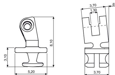
90° PLASTIC HINGE 03FRC4140A2BN0
