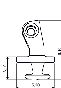
90° PLASTIC HINGE 03FRC4138A2BN0
