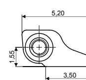
SOLDERING HINGE 03FRC4550A1BY0
