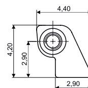
STEP HINGE 03FRC4162A1BY0
