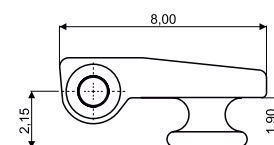
180° PLASTIC HINGE 03FRC4145A2BN0
