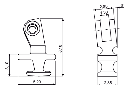
90° PLASTIC HINGE 03FRC4136A2BN0
