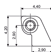
STEP HINGE 03FRC4161A1BY0
