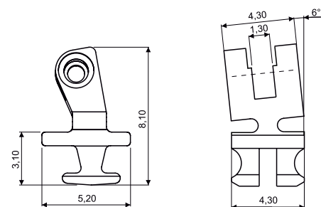
90° PLASTIC HINGE 03FRC4142A2BN0
