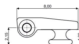
180° PLASTIC HINGE 03FRC4146A2BN0
