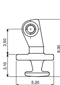
90° PLASTIC HINGE 03FRC4137A2BN0
