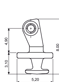
90° PLASTIC HINGE 03FRC4139A2BN0
