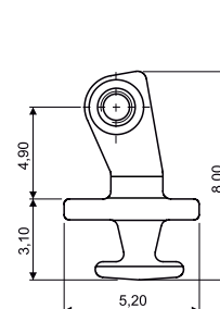
90° PLASTIC HINGE 03FRC4141A2BN0
