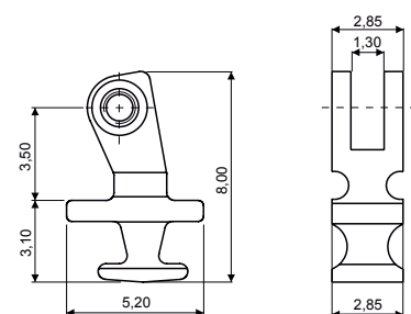
90° PLASTIC HINGE 03FRC4135A2BN0
