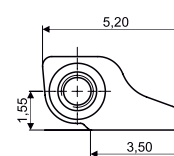
SOLDERING HINGE 03FRC4552A1BY0
