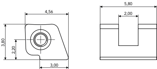
SOLDERING HINGE 03FRC2868A1BY0
