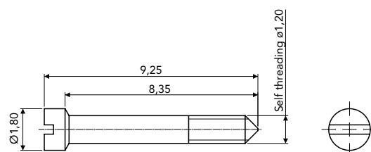
SELF THREADING SCREW 07V118092500 Material: Stainless steel
