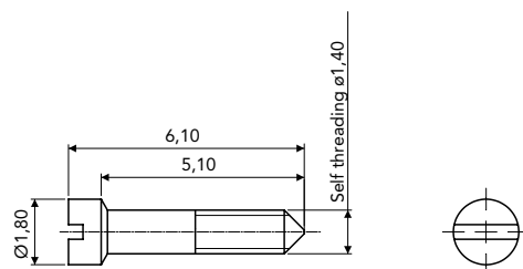
SELF THREADING SCREW 07VIA0366A1BYX Material: Stainless steel
