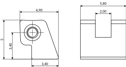
SOLDERING HINGE 03FRC2867A1BY0
